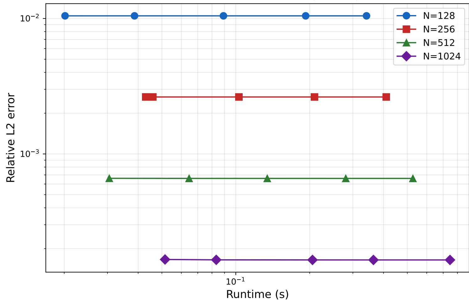
Relative L2 error vs runtime (all runs)
