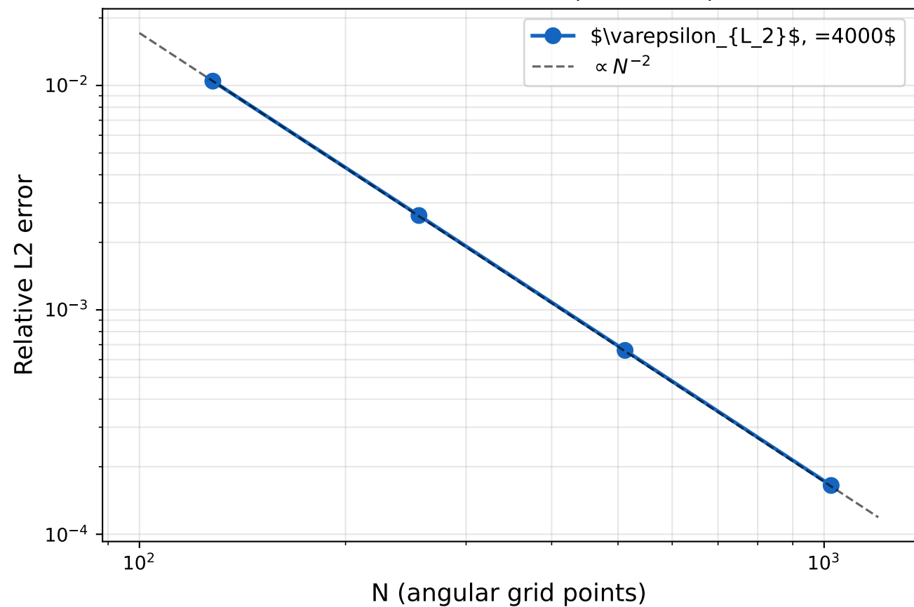
Relative L2 error vs N (Nt = 4000)
